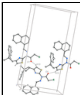
Fig. 2. Part of the crystal structure of the title compound, showing the C—H...O hydrogen bonding. For clarity, only H atoms involved in hydrogen bonding have been included. For symmetry codes, see Table 1.
