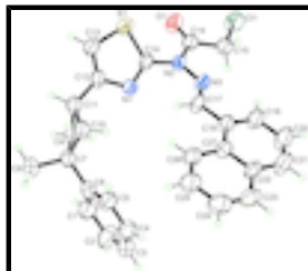
Fig. 1. An ORTEP-3 (Farrugia, 1997) drawing of (I), showing the atomic numbering scheme. Displacement ellipsoids are drawn at the 30% probability level.
