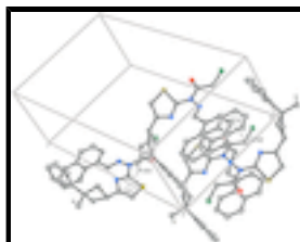
Fig. 3. Part of the crystal structure of the title compound, showing the C—H... \pi interactions. For clarity, only H atoms involved in hydrogen bonding have been included. For symmetry codes, see Table 1.
